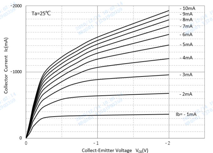
Static Characteristic
