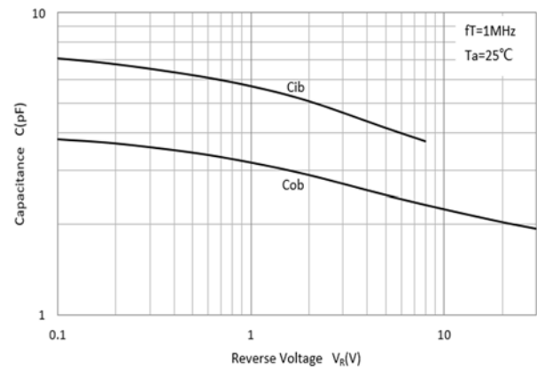
Fig 6: C_{ob}/C_{ib}-V_{CB}/V_{EB}
