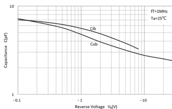
Fig 6: Cob/Cib- V_{CB}/V_{EB}
