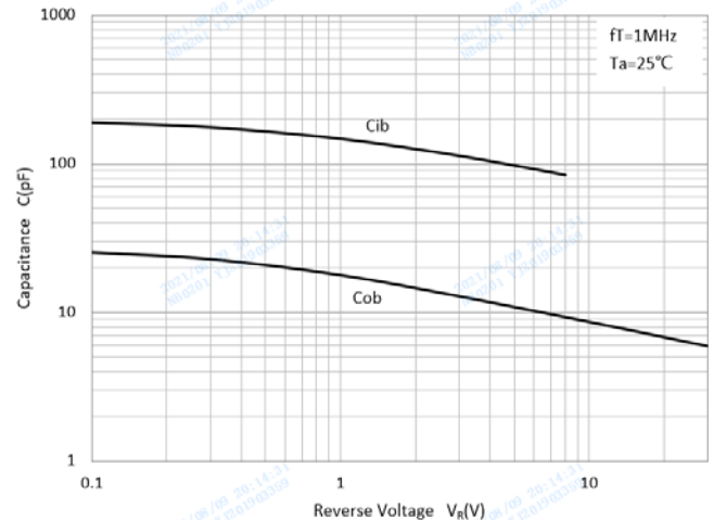
C_{ob}/C_{ib}-V_{CB}/V_{EB}
