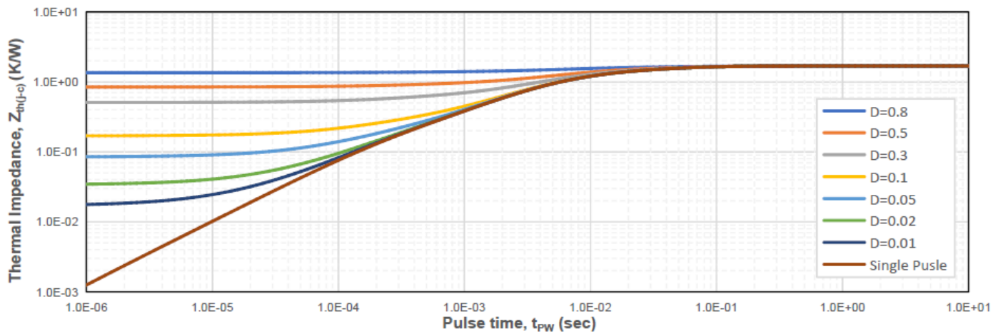
Figure 21. Transient Junction to Case Thermal Impedance
