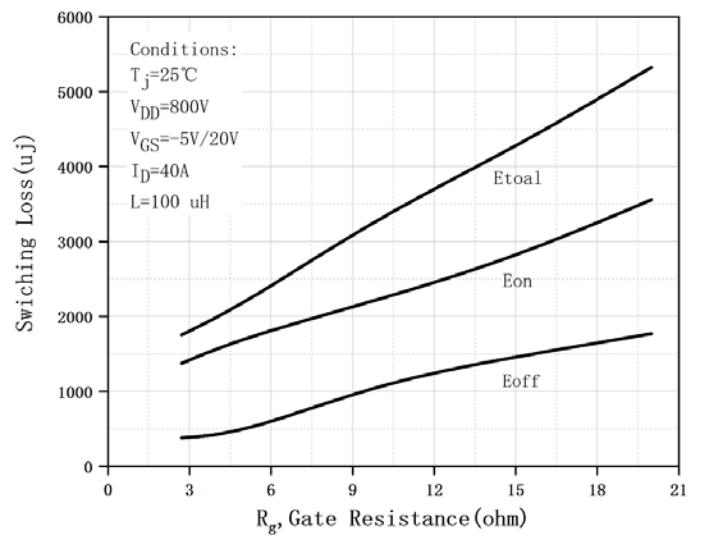
Figure 18. Clamped Inductive Switching Energy vs. External Gate Resistor
