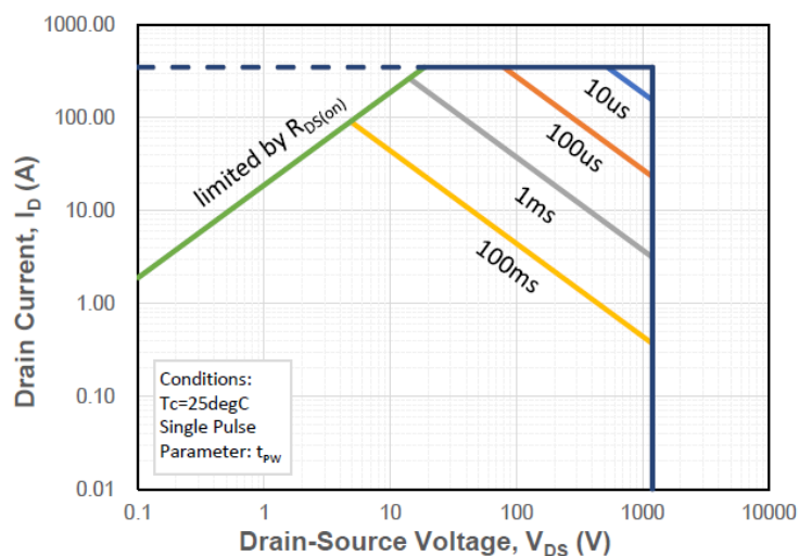
Figure 15. Safe Operating Area
