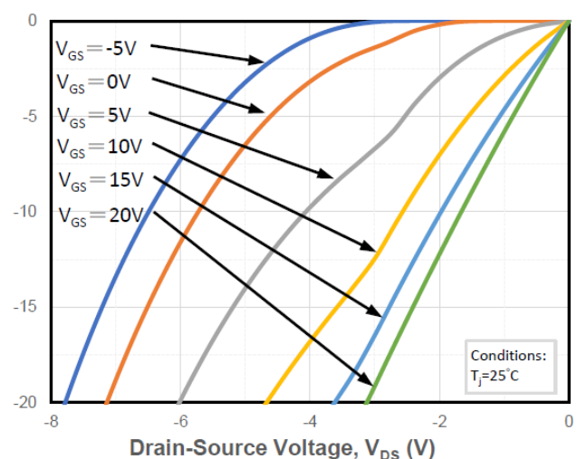
Figure 8. Reverse Output Characteristics at T_J = 25^\circ\text{C}
