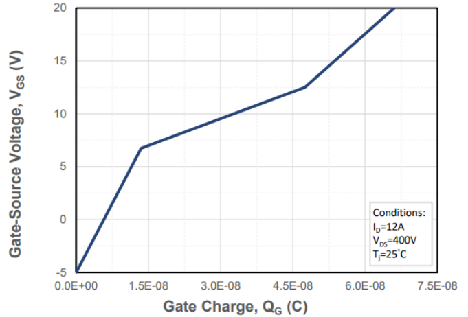
Figure 16. Gate Charge Characteristics
