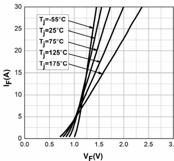
Figure 1. Forward Characteristics
