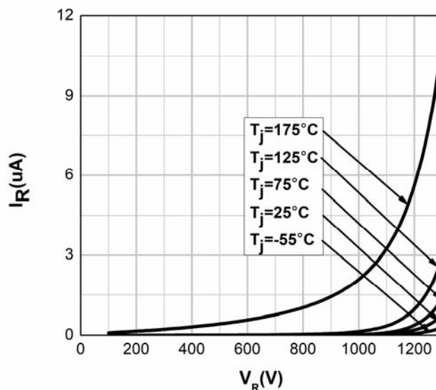
Figure2. Reverse Characteristic
