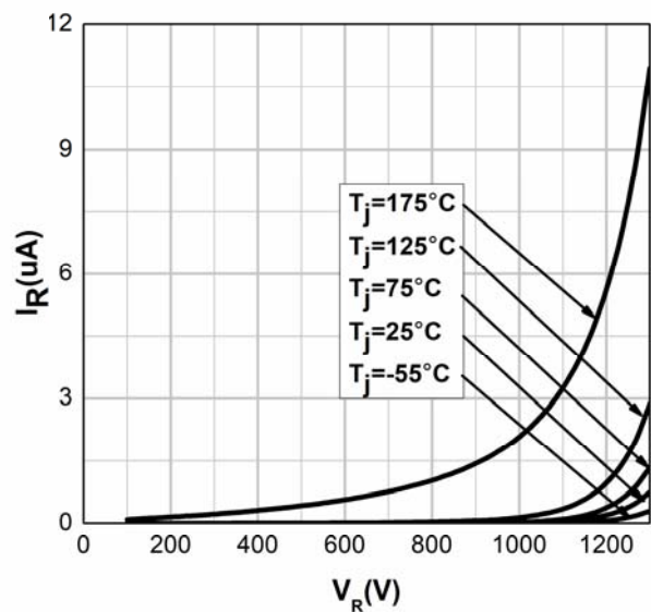
Figure 2. Reverse Characteristics
