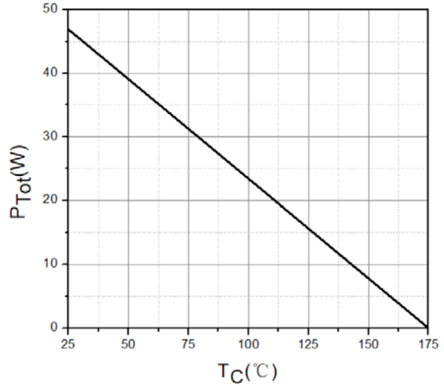
Figure 6. Power Derating
