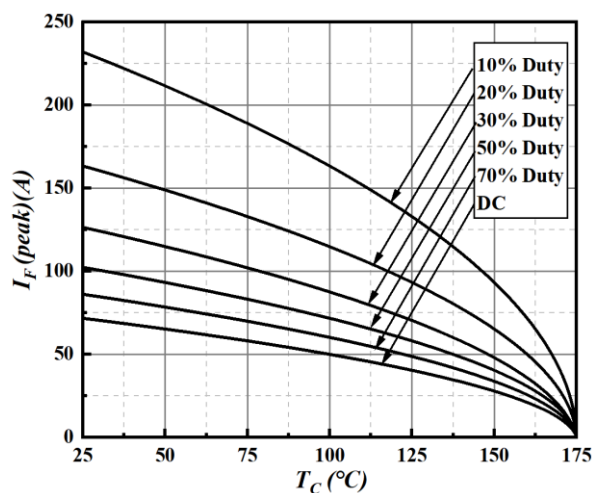
Fig7. Current Derating
