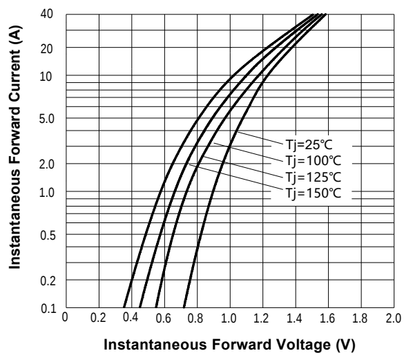
FIG3: Forward Voltage
