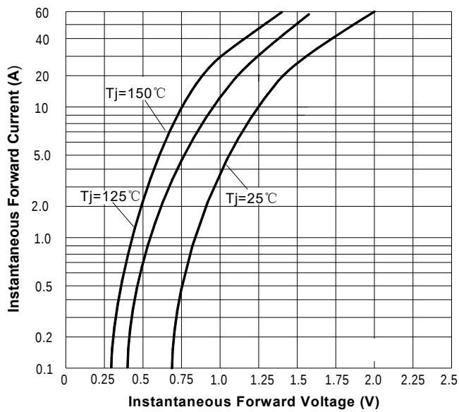
FIG3: Forward Voltage
