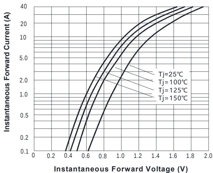
FIG3: Forward Voltage
