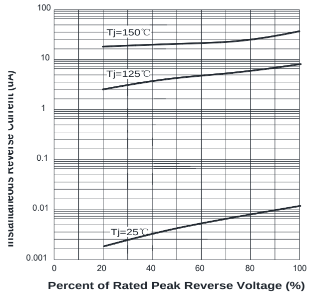
FIG4: Instantaneous Reverse Characteristic
