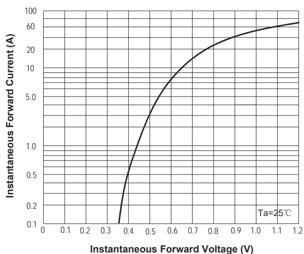
FIG3: Forward Voltage
