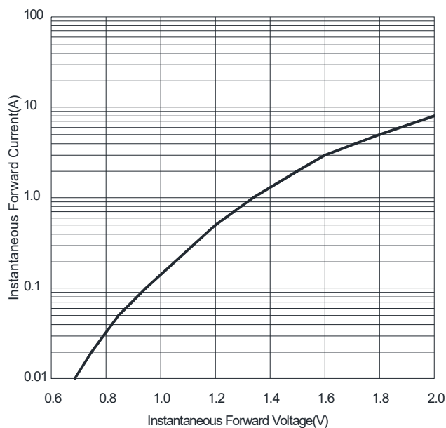
FIG3: Forward characteristics
