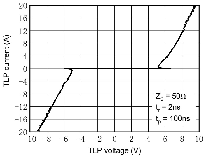
Fig.9 TLP Measurement
