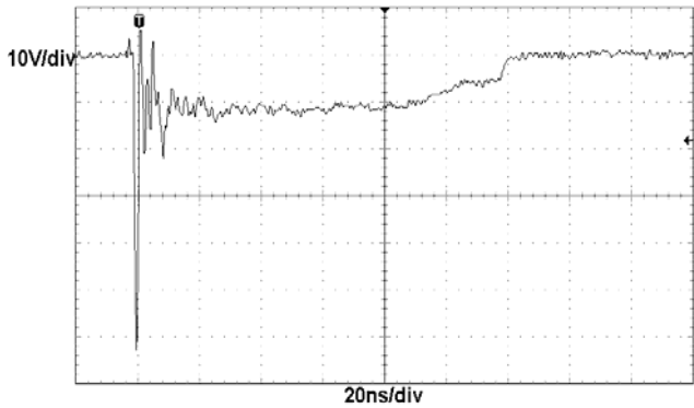
(-8kV contact discharge per IEC61000-4-2)
