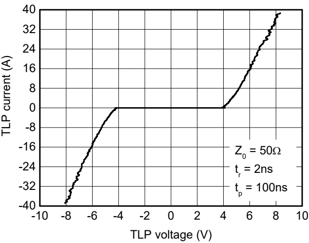
TLP Measurement
