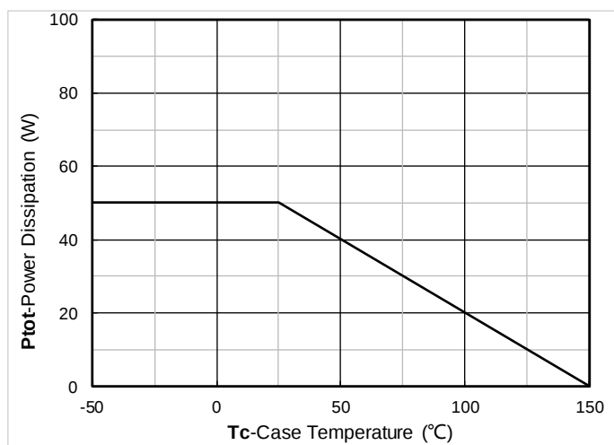
Figure 11. Power dissipation
