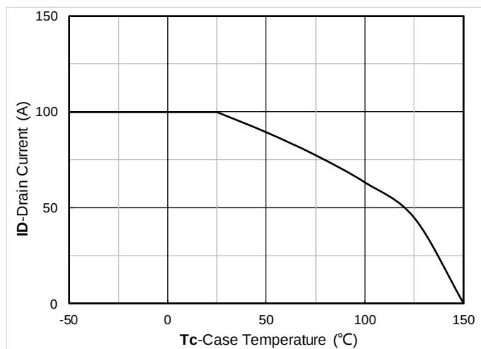
Figure 10. Current dissipation
