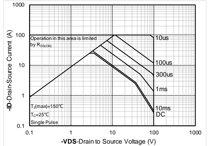
Figure8.Safe Operation Area
