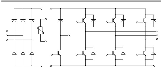
Circuit
