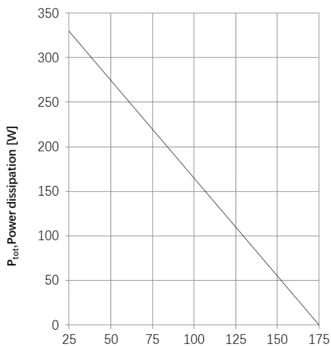
Fig1. Power dissipation as a function of case temperature ( T_j \leq 175^\circ\text{C} )
